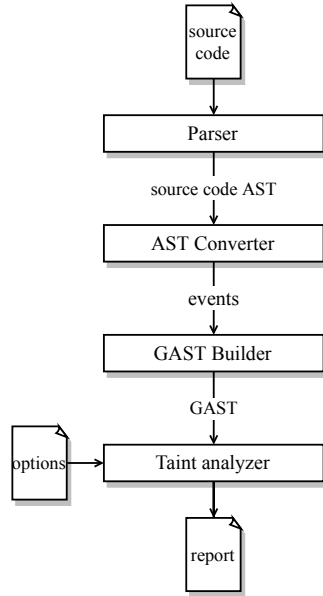
Figure 1: GT - data flow and architecture overview
