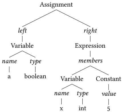
Figure 2: GAST resulting from executing listing 5
